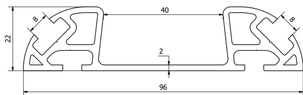
MONORAIL 40 mm
