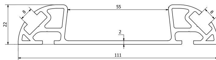
MONORAIL 55 mm
