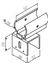
SLIDE MOUNT-G
