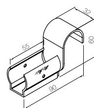
SLIDE MOUNT-D
